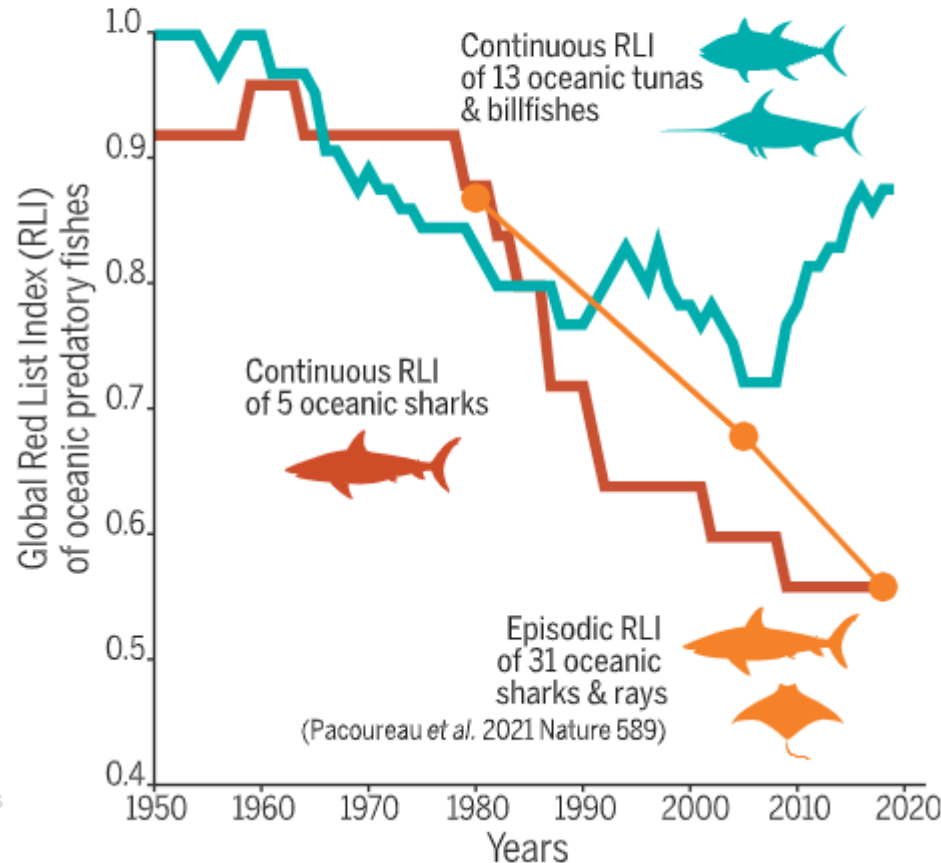
B Trajectory of the extinction risk in oceanic predatory fishes since 1950 for tracking progress towards global sustainability and biodiversity targets
